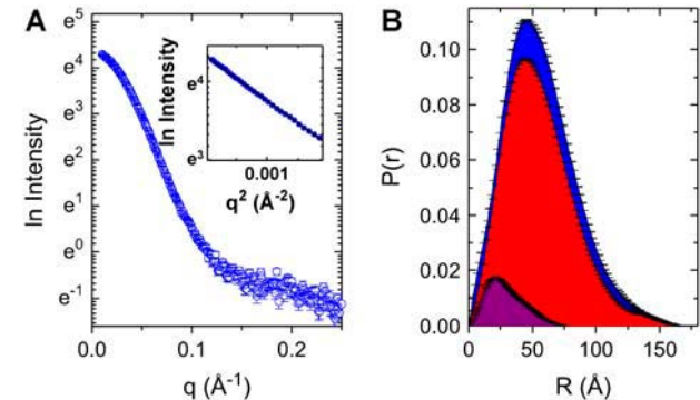
FIGURE 2 (A) SAXS data for the 1.3:1 mixture of sCD4/gp120. Inset shows the linearity of the Guinier plot. (B) A comparison of the P(r) curves calculated from the SAXS data for the unliganded gp120 (red), sCD4 (purple), and their mixture (blue).
